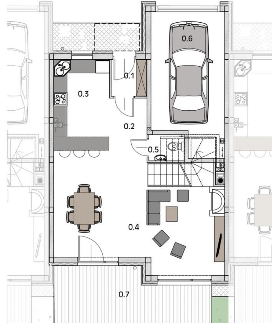
Parter
